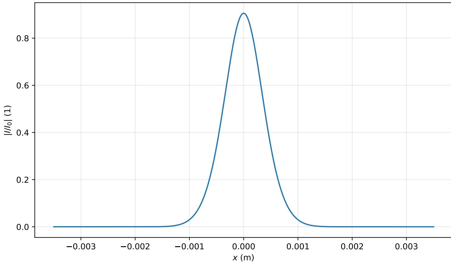
Intensity profile I(x, y = 0, z = 1.115m)/I_0 , P_{in}=0.3P_{cr} , artificial time
